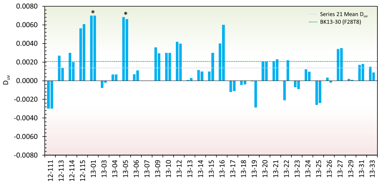
Figure 5. D_{uv} for both samples of each Series 21 linear LED lamp. The two products shown with an asterisk did not meet the ANSI criterion for nominally white light.
