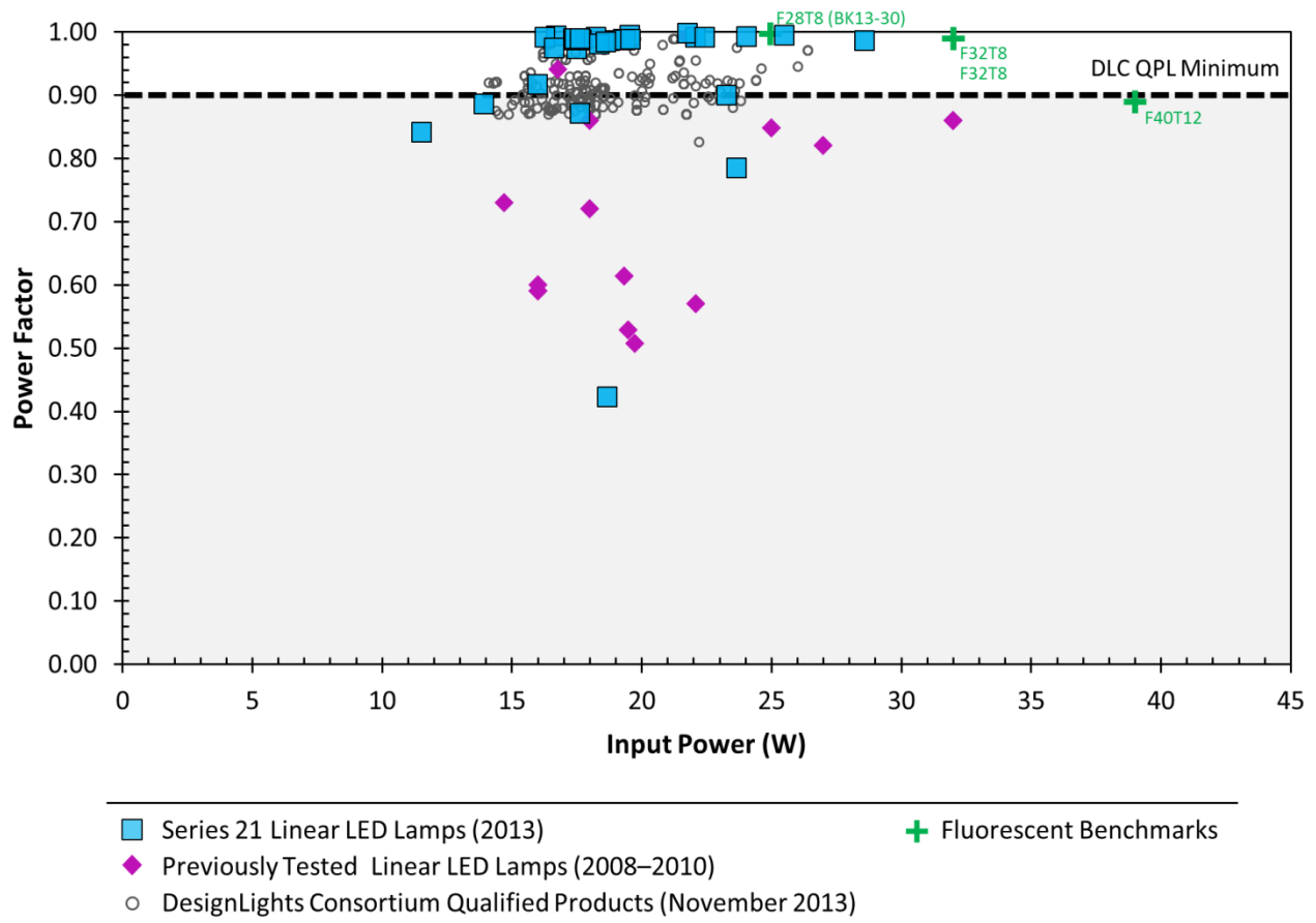
Figure 6. Power factor and input power characteristics of the Series 21 products and auxiliary data sets.
