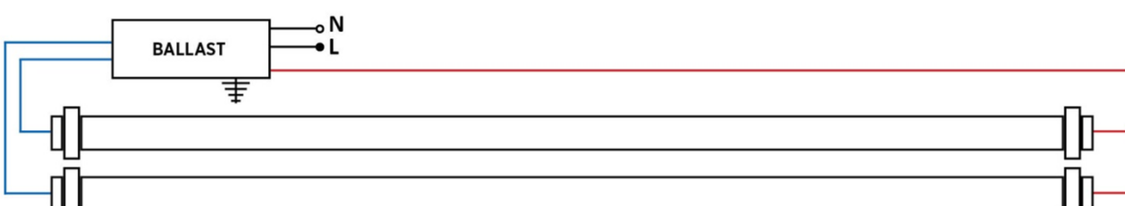
F. Existing Instant-Start electronic ballast (shunted sockets)
