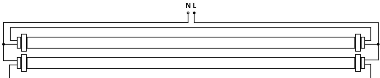
Figure F1. Typical wiring diagrams for LED T8s with an internal driver.
