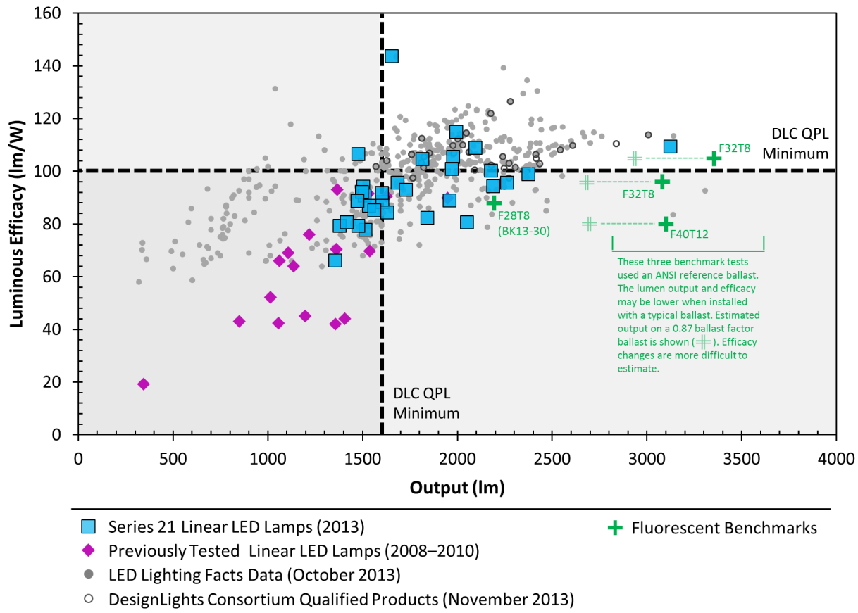
Figure 2. Luminous efficacy versus lumen output for the Series 21 linear LED lamps compared to other datasets. Compared to earlier CALiPER testing, many of the Series 21 lamps demonstrated higher lumen output and higher efficacy. However, few exceeded the efficacy of CALiPER-tested F32T8 benchmarks by a substantial amount.
