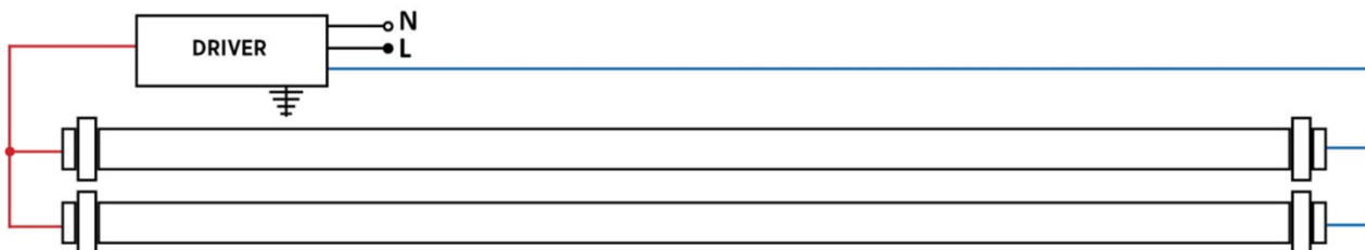
E. Remote driver, double-ended wiring (shunted sockets)
