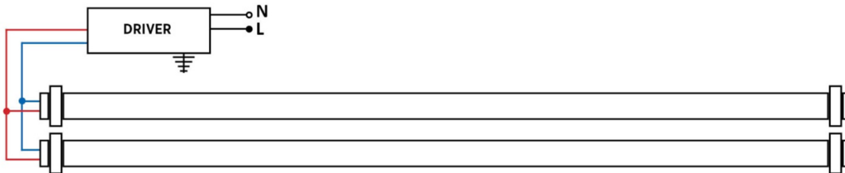
D. Remote driver, single-ended wiring (unshunted sockets)
