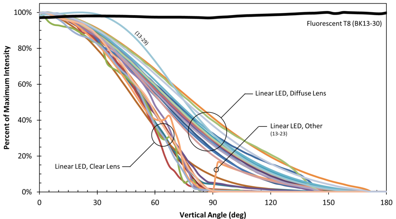
Figure 3. Relative luminous intensity distribution of the Series 21 products (90° horizontal plane). Although none of the LED products were close to matching the fluorescent benchmark—which had relatively uniform intensity at all vertical angles—the data did reveal a distinct difference between lamps with a clear lens and lamps with a frosted lens. The beam angle is twice the vertical angle at which the intensity is 50% of maximum intensity (ANSI/IES RP-16-10), assuming symmetry.
